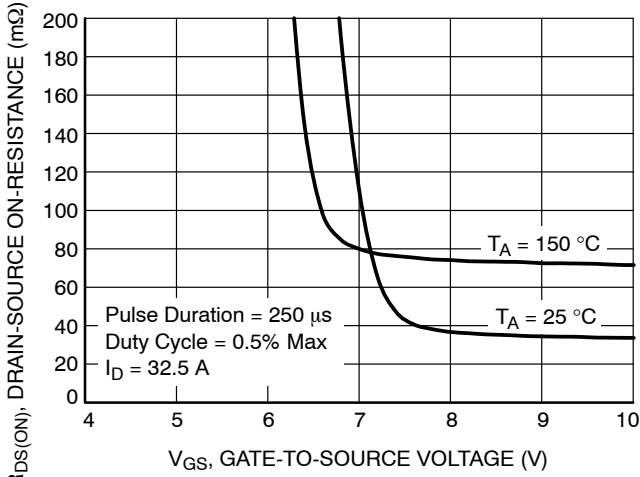
Figure 16. R_{DS(ON)} vs. Gate Voltage
