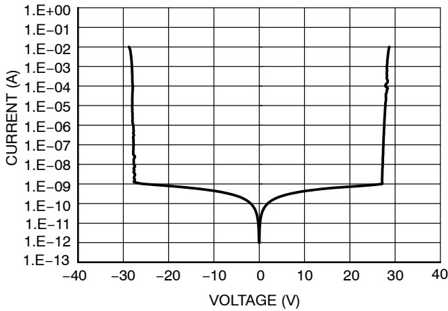
Figure 2. IV Characteristics
