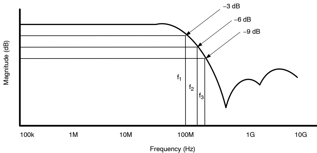
Figure 8. Filter Bandwidth
