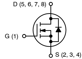
N-CHANNEL MOSFET
