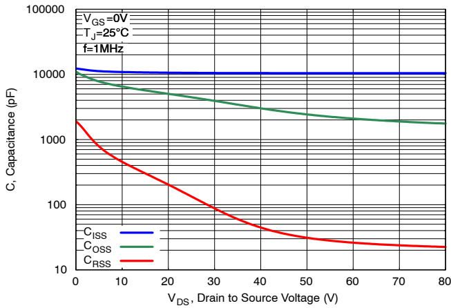
Figure 7. Capacitance Characteristics
