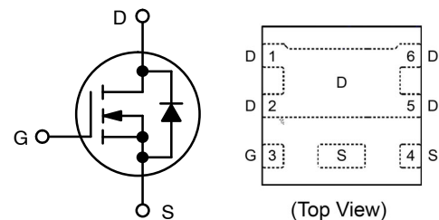
N-CHANNEL MOSFET
