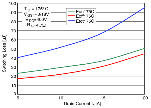
Figure 16. Switching Loss vs. Drain Current
