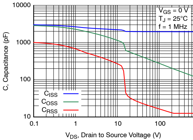
Figure 7. Capacitance Characteristics
