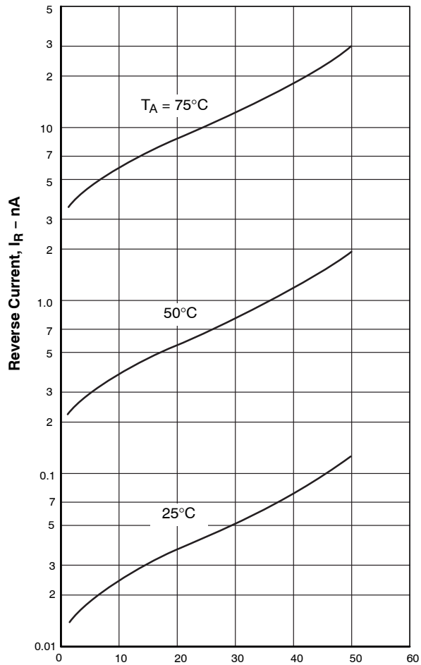
Reverse Voltage, V_R – V
