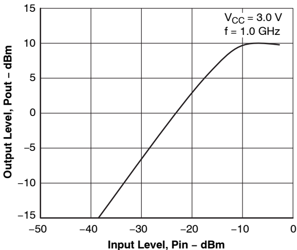
Figure 8. P_{out} - P_{in}
