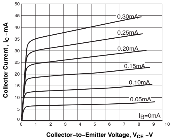
Figure 1. I_C - V_{CE}
