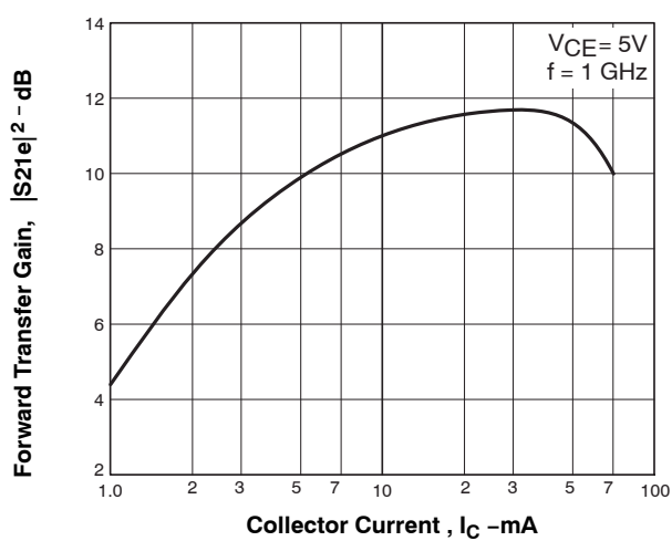
Figure 8. |S_{21e}|^2 – I_C
