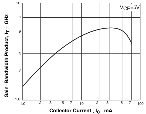
Figure 4. f_T - I_C
