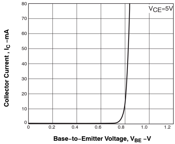
Figure 2. I_C - V_{BE}
