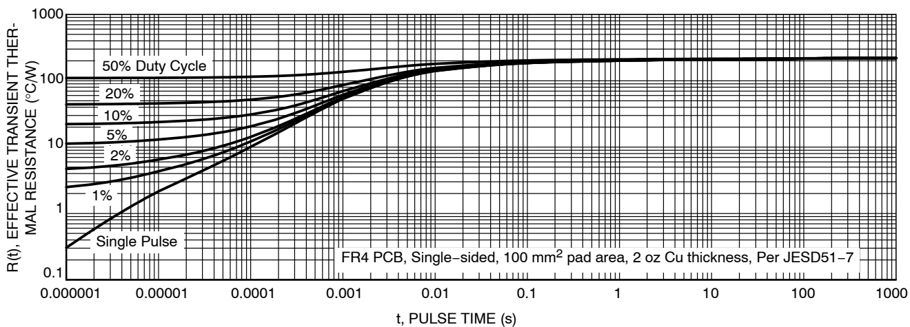
Figure 14. Thermal Resistance
