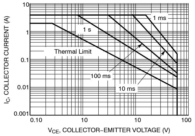
Figure 8. Safe Operating Area Single Pulse Test @ T_{amb} = 25\text{ °C}
