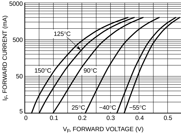
Figure 5. Forward Voltage
