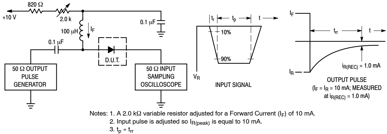
Figure 1. Recovery Time Equivalent Test Circuit
