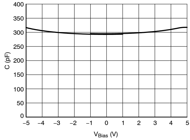
Figure 7. CV Characteristics
