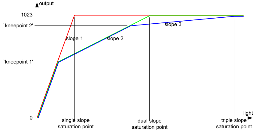
Figure 24. Multiple Slope Operation
