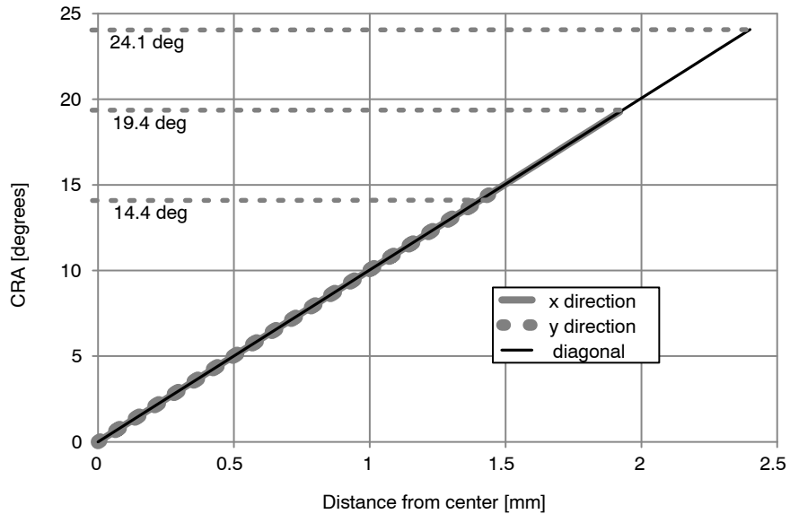
Figure 8. Variation of Peak Responsivity Angle (CRA) as a Function of Distance from the Center of the Array (High CRA Version)
