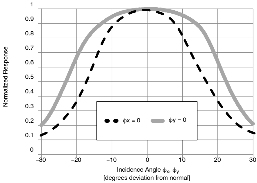
Figure 7. Central Pixel Photoresponse to a Fixed Optical Power with Incidence Angle varied along \phi_x and \phi_y (High CRA Version)
