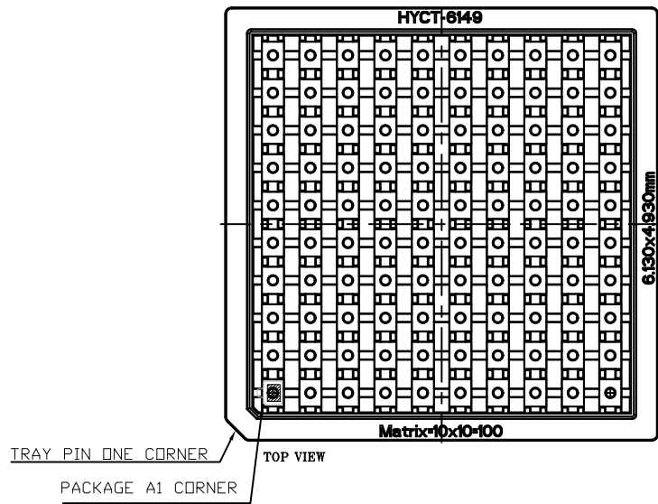
Figure 45. Pin 1 Location
