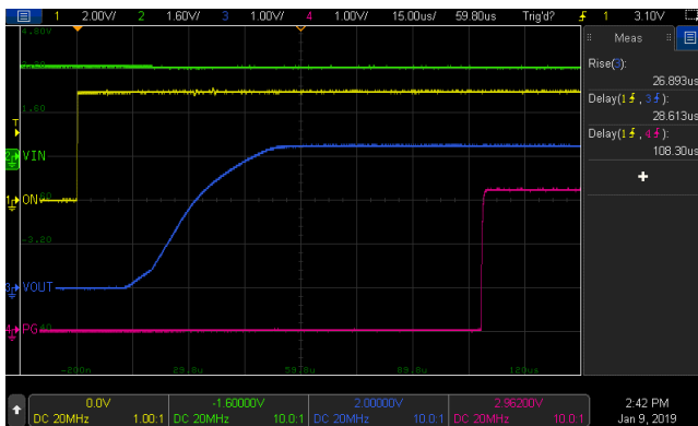
Figure 31. Turn-on Response
