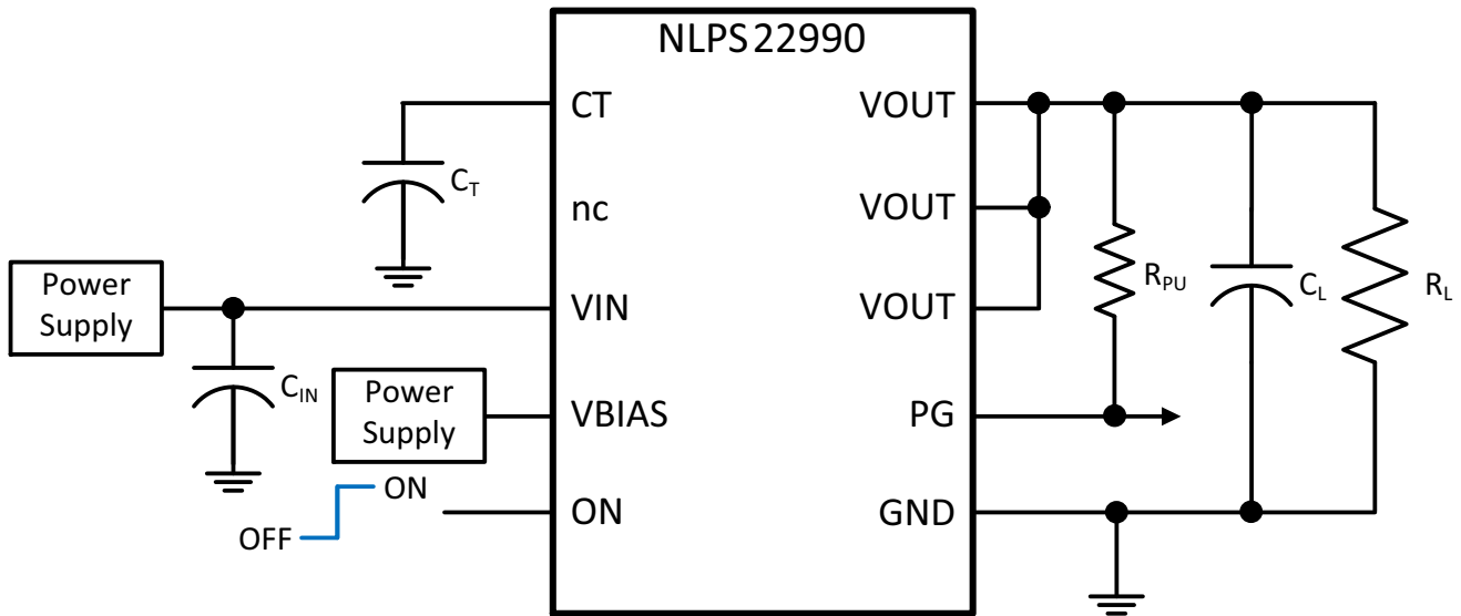
Figure 38. Timing Test Circuit
