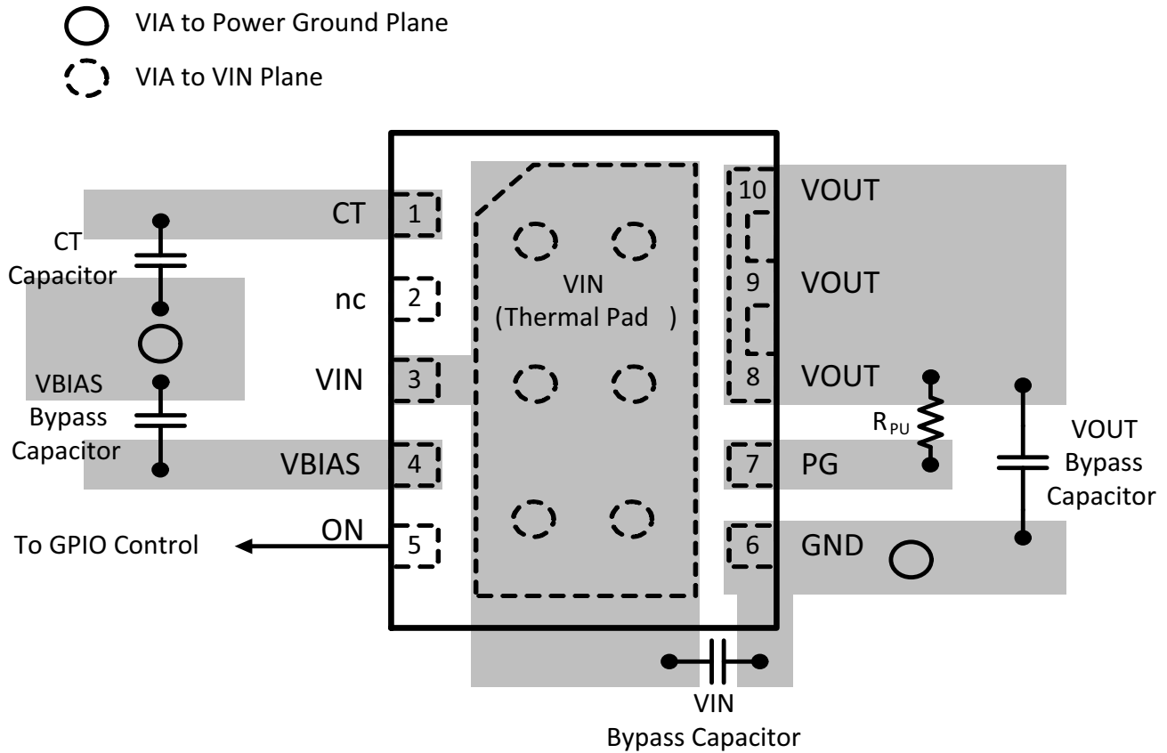
Figure 43. Layout Example
