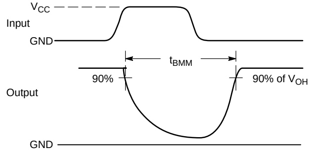
Figure 6. t_{BBM} (Time Break-Before-Make)
