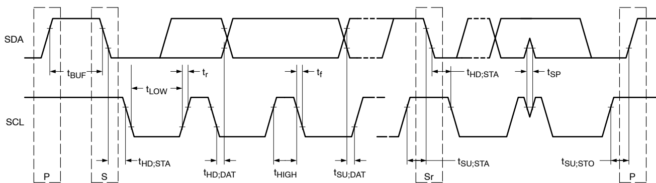
Figure 16. Definition of Timing on the I 2 C Bus
