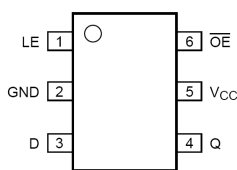
Figure 1. SC88 (Top View)
