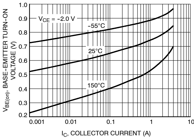
Figure 14. Base Emitter Turn-On Voltage vs. Collector Current
