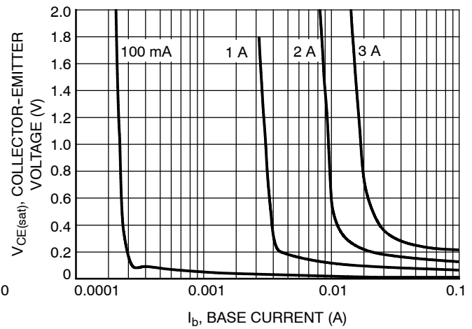
Figure 15. Saturation Region
