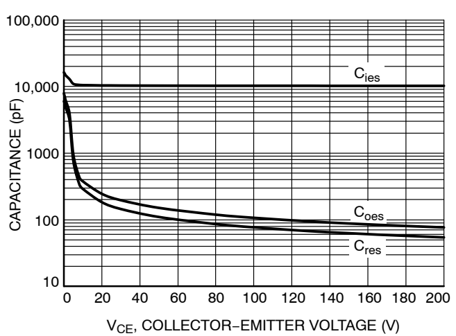
Figure 6. Typical Capacitance
