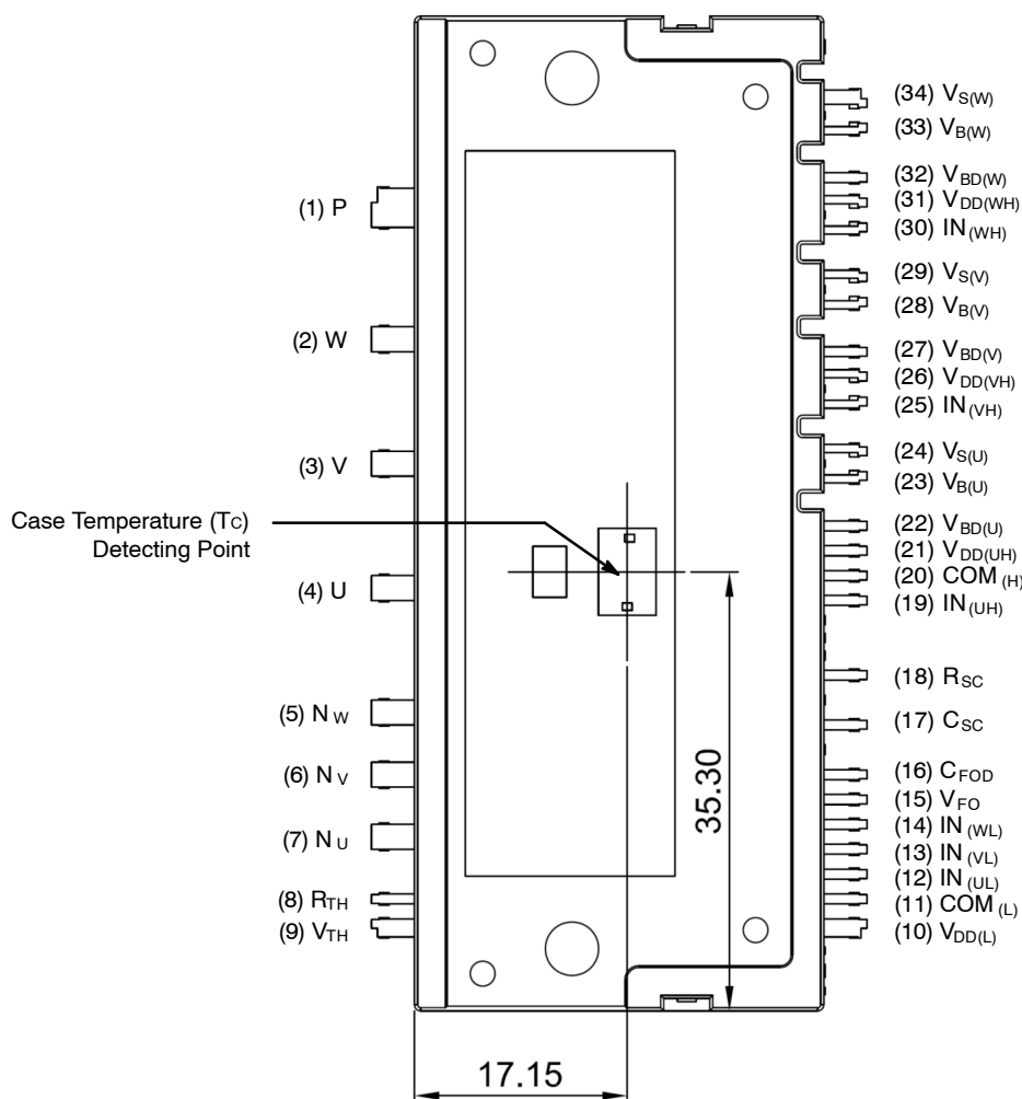
Figure 1. Pin Configuration – Top View
