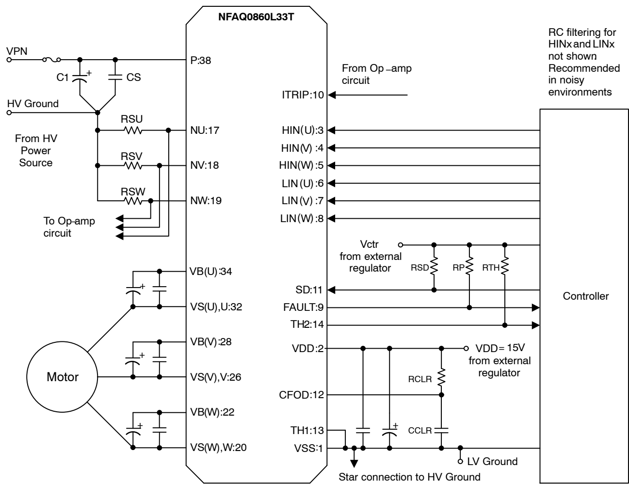
Figure 2. Application Schematic
