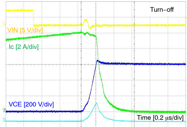
Figure 24. Turn-off Switching Waveform
