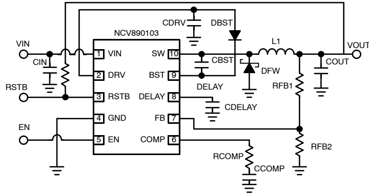
Figure 1. Typical Application
