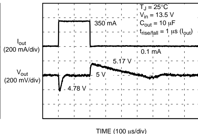
Figure 30. Load Transients
