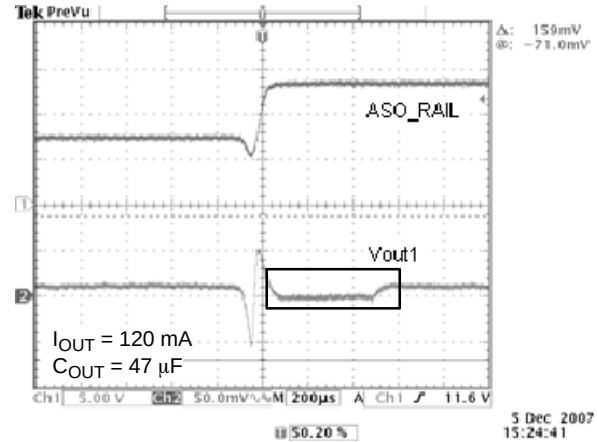
Figure 3. V OUTX Response to ASO Switchover Event
