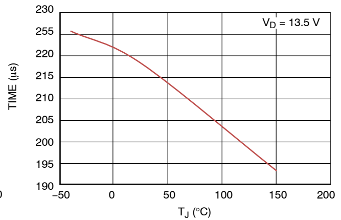
Figure 49. Turn On Delay CL Mode vs. T_J
