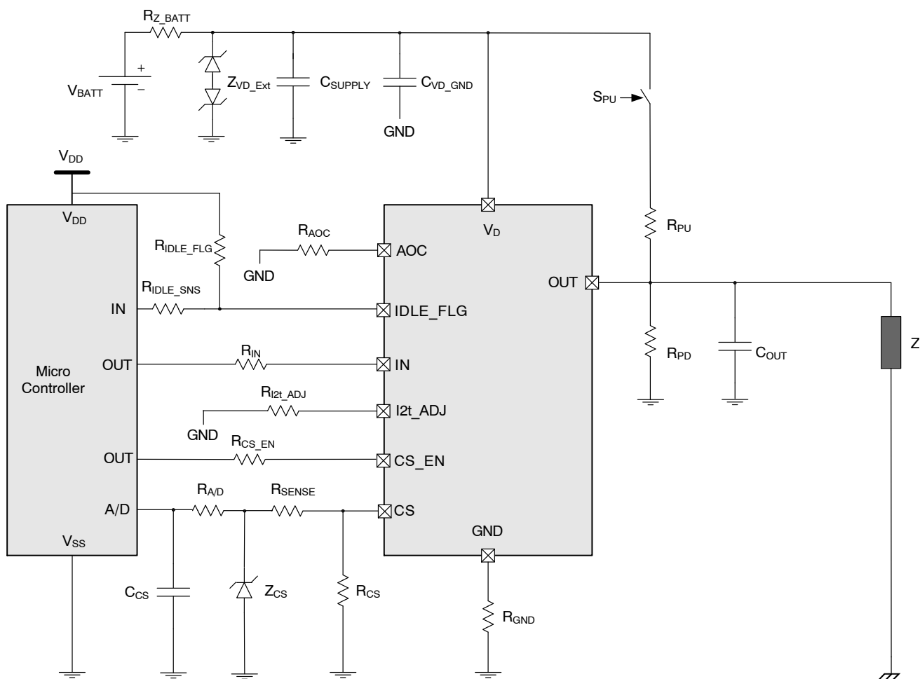
Figure 4. Application Diagram
