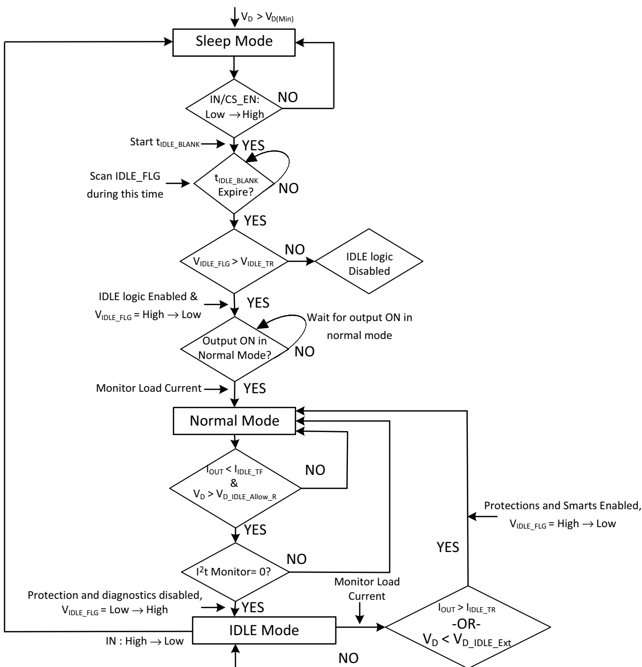
Figure 8. NCV84006G IDLE Mode Flowchart
