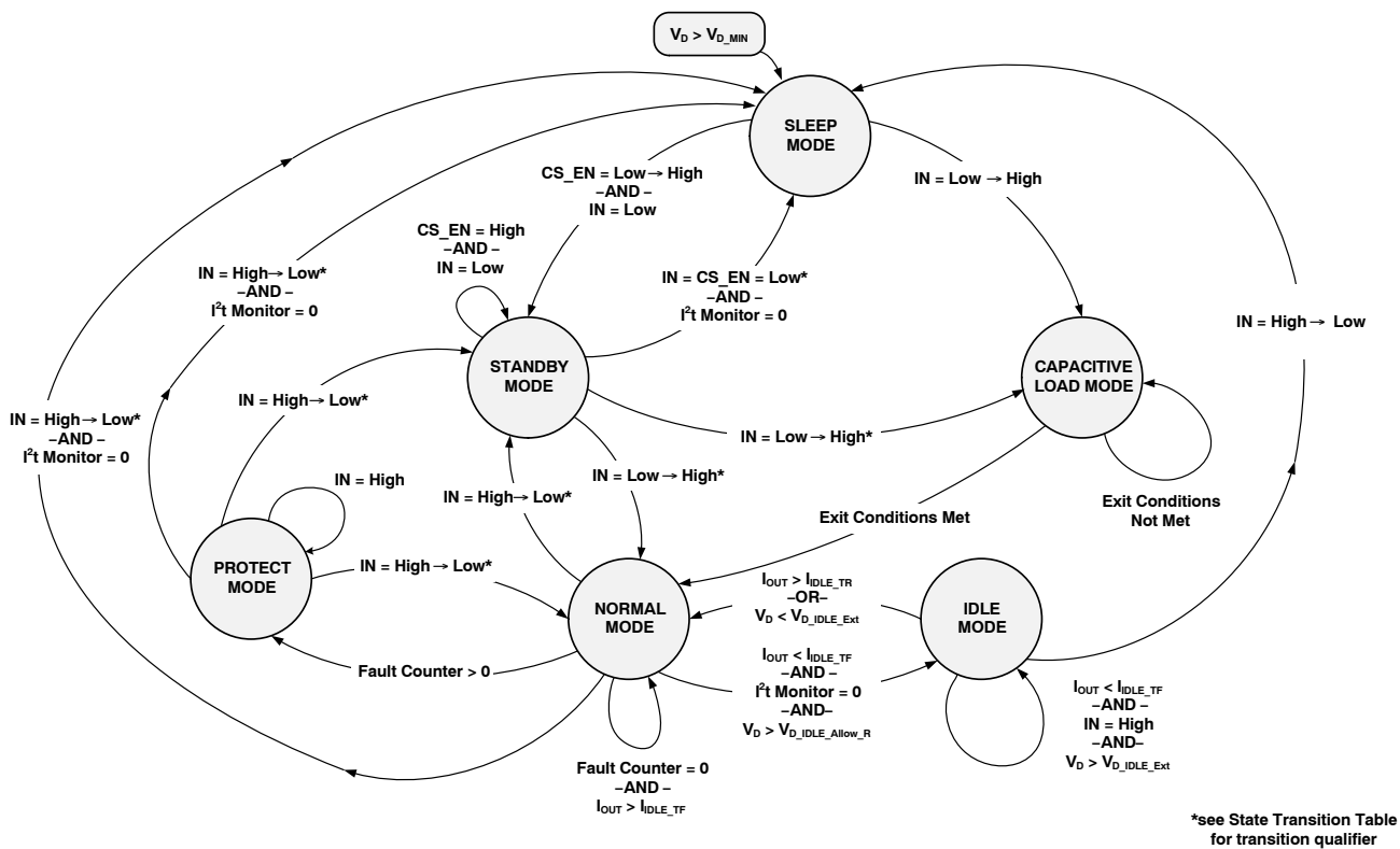
Figure 5. NCV84006G Operation Modes and Transitions
