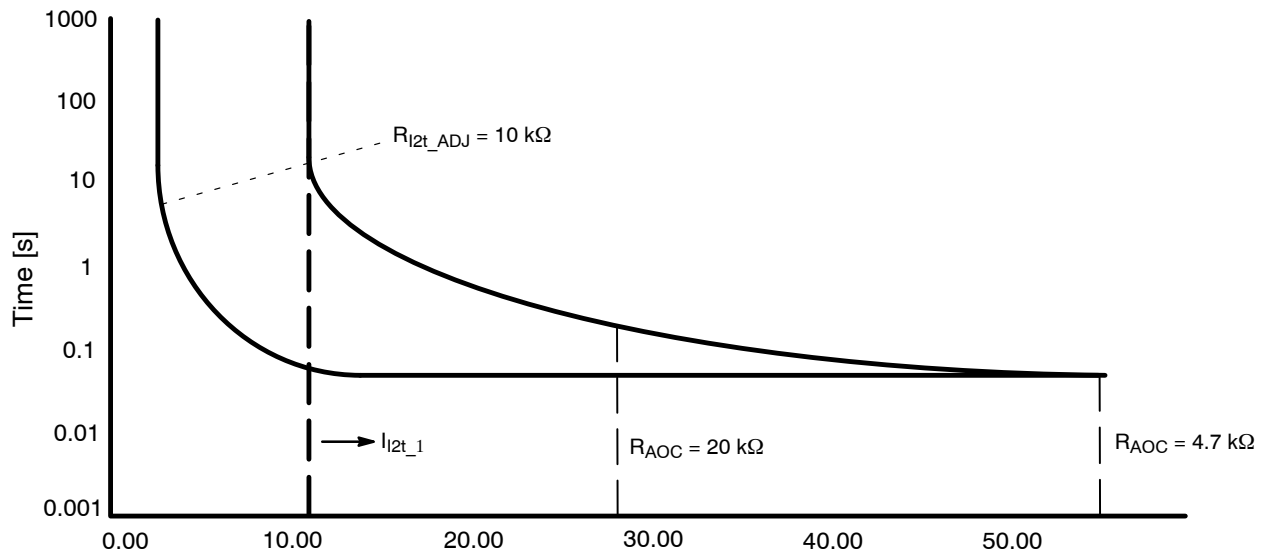
Figure 26. I^2t Maximum Overcurrent Adjustability
