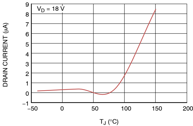
Figure 42. Quiescent Current vs. T_J
