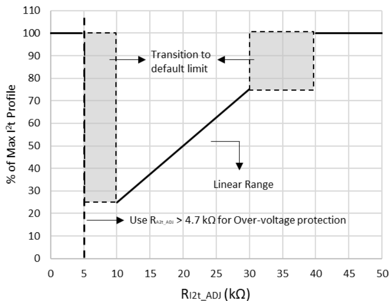
Figure 24. Adjustable I 2 t Profiles vs R I2t_ADJ
