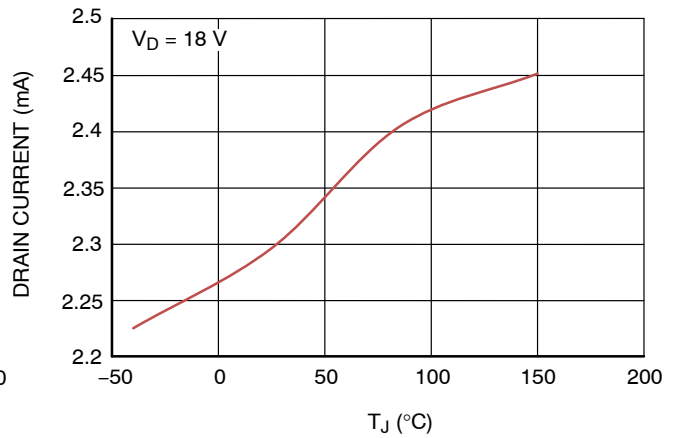
Figure 43. Quiescent Current, Diagnostic Active vs. T_J
