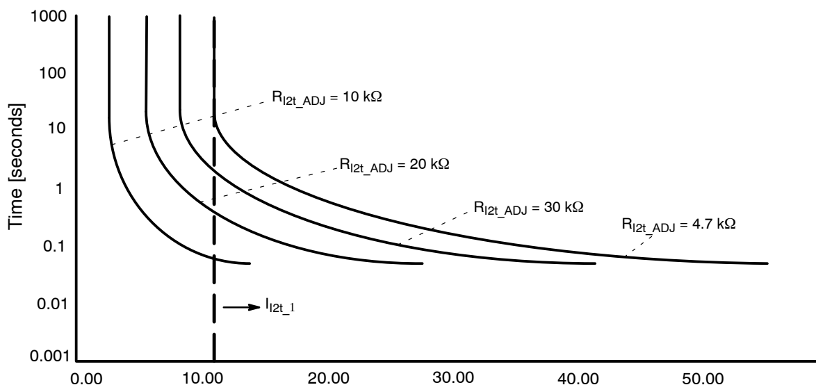
Figure 25. I 2 t Protection Implementation
