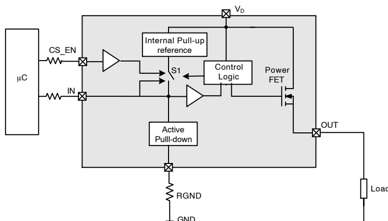
Figure 9. NCV84006G IN Latch Operational Diagram
