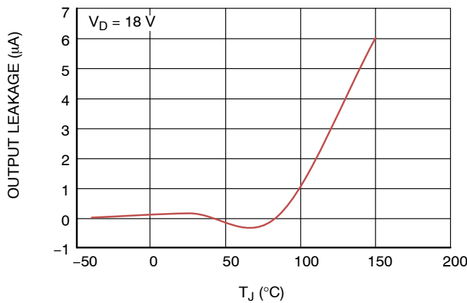
Figure 44. Output Leakage vs. T_J
