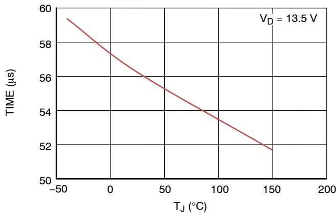
Figure 48. Turn On Time Normal Mode vs. T_J
