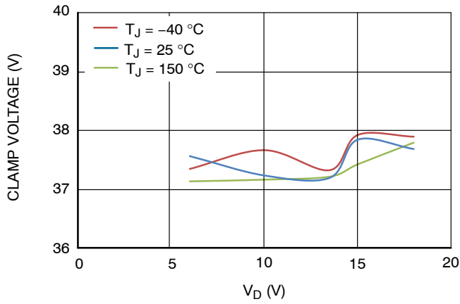
Figure 52. Drain-to-Source Clamping vs. T_J
