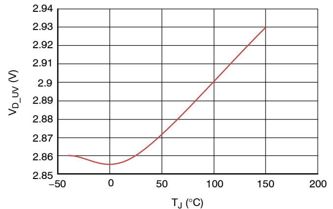
Figure 51. Undervoltage Shutdown (Turn-Off) vs. T_J
