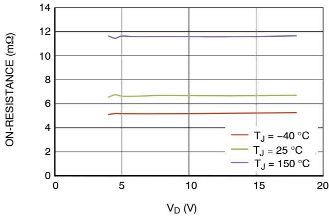
Figure 40. On-Resistance vs. V_D
