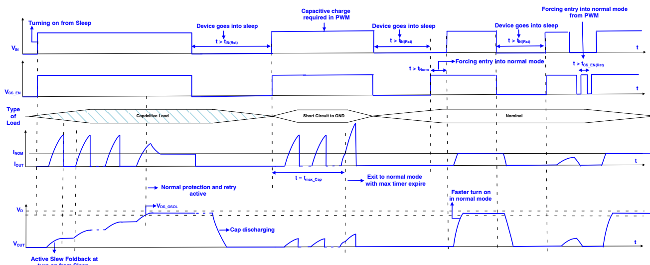
Figure 12. Capacitive Load Inrush Management
