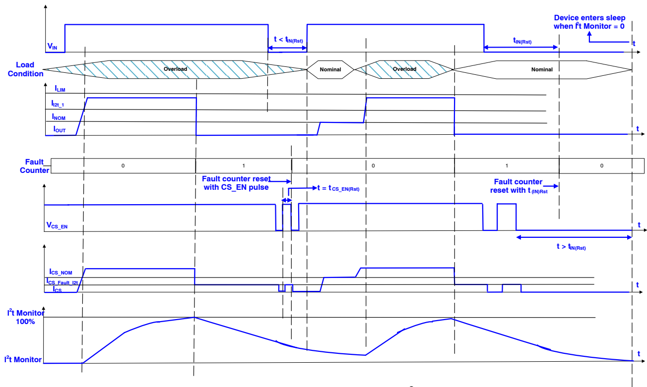
Figure 29. Retry Strategy in Case of I^2t Fault
