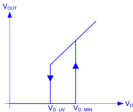
Figure 17. Under-voltage Behavior
