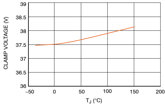
Figure 54. Overvoltage Clamp vs. T_J
