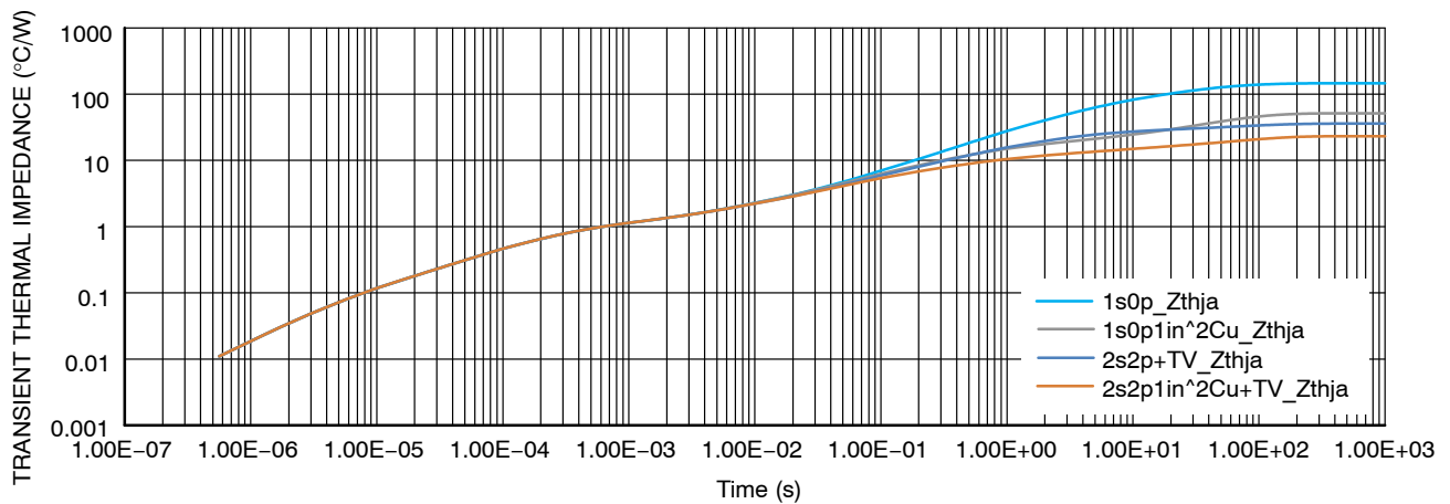
Figure 55. Transient Thermal Response
