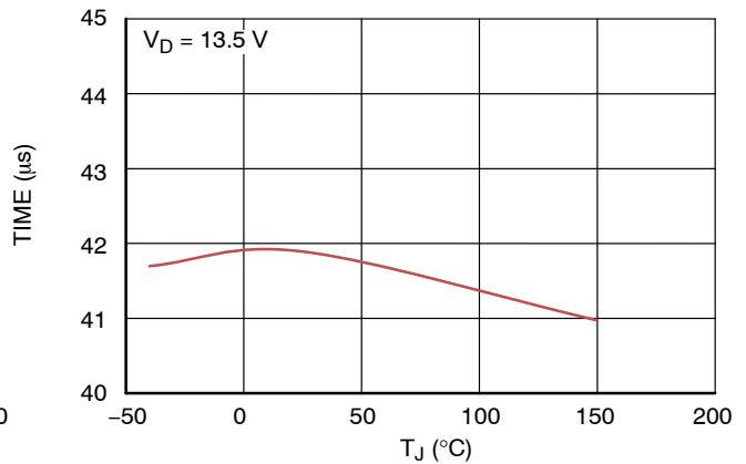
Figure 45. Turn Off Delay vs. T_J
