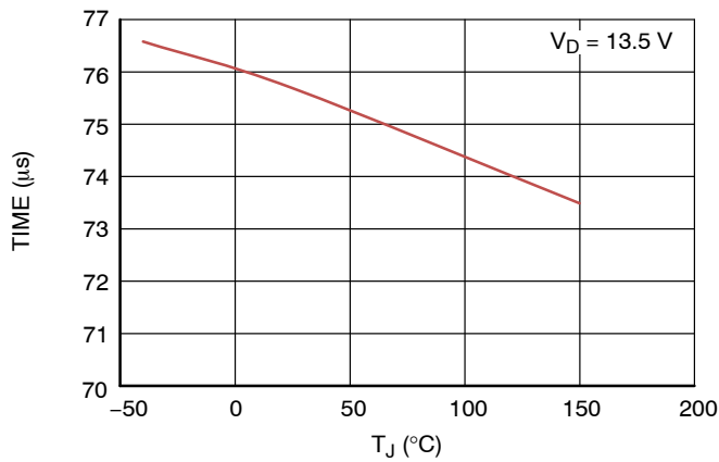
Figure 46. Turn Off Time vs. T_J
