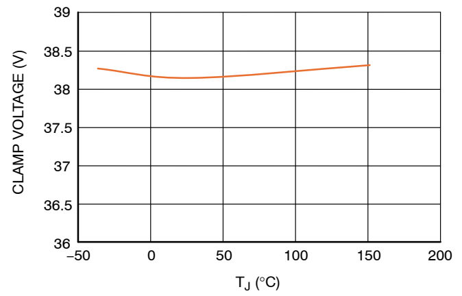
Figure 53. CS Clamp vs. T_J
