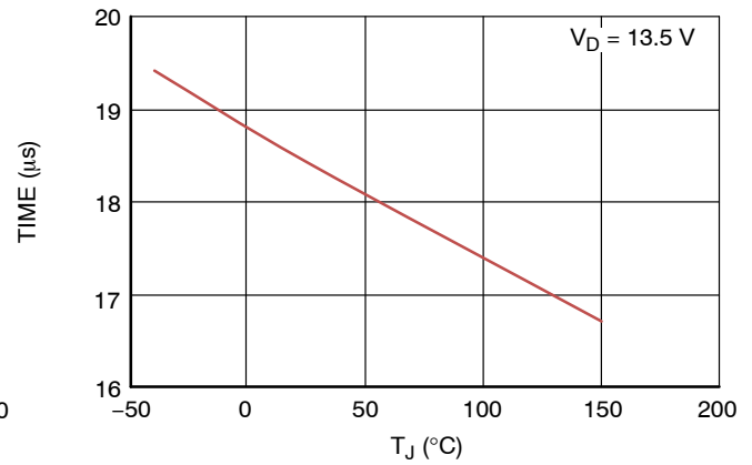
Figure 47. Turn On Delay Normal Mode vs. T_J
