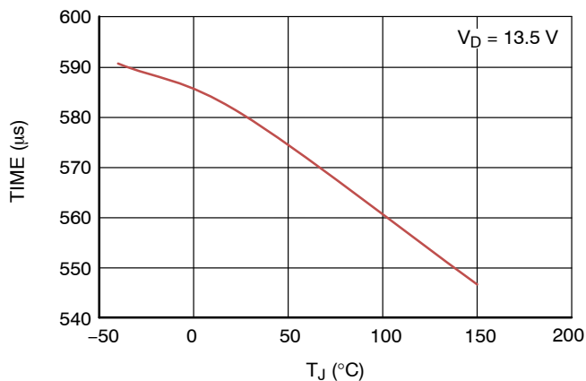
Figure 50. Turn On Time CL Mode vs. T_J
