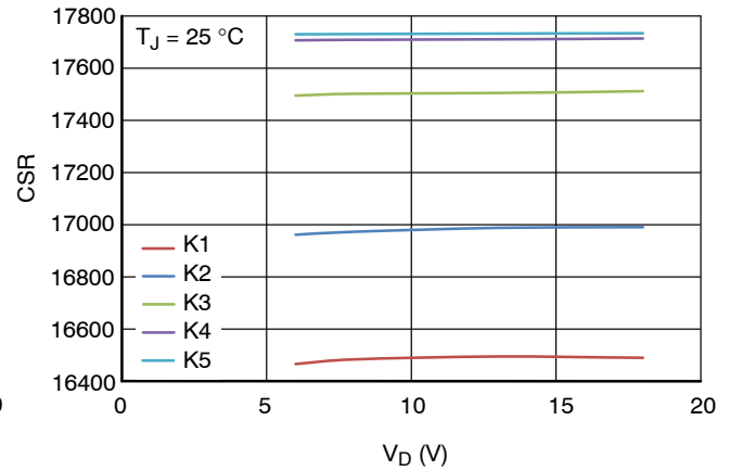
Figure 41. Current Sense Ratio vs. V_D
