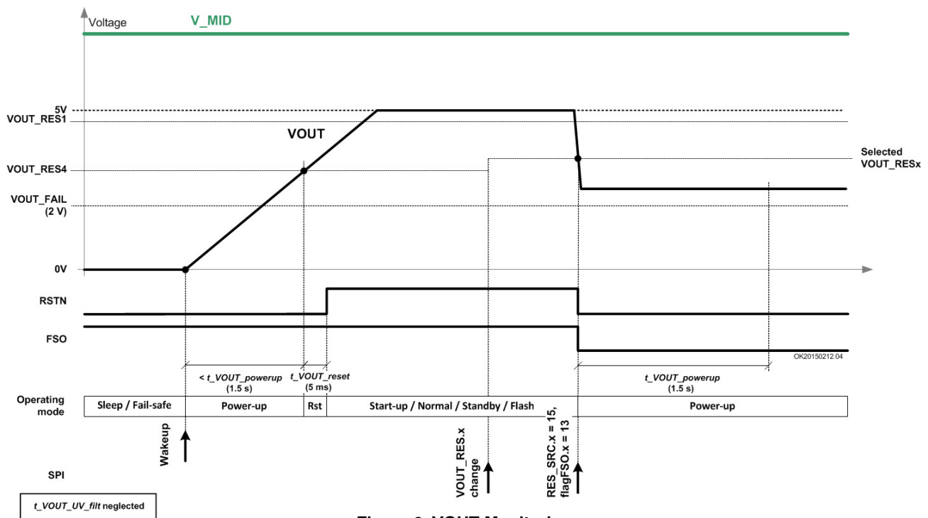
Figure 6. VOUT Monitoring
