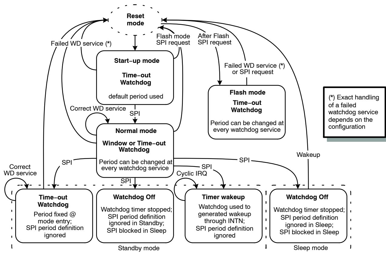
Figure 14. Watchdog Modes
