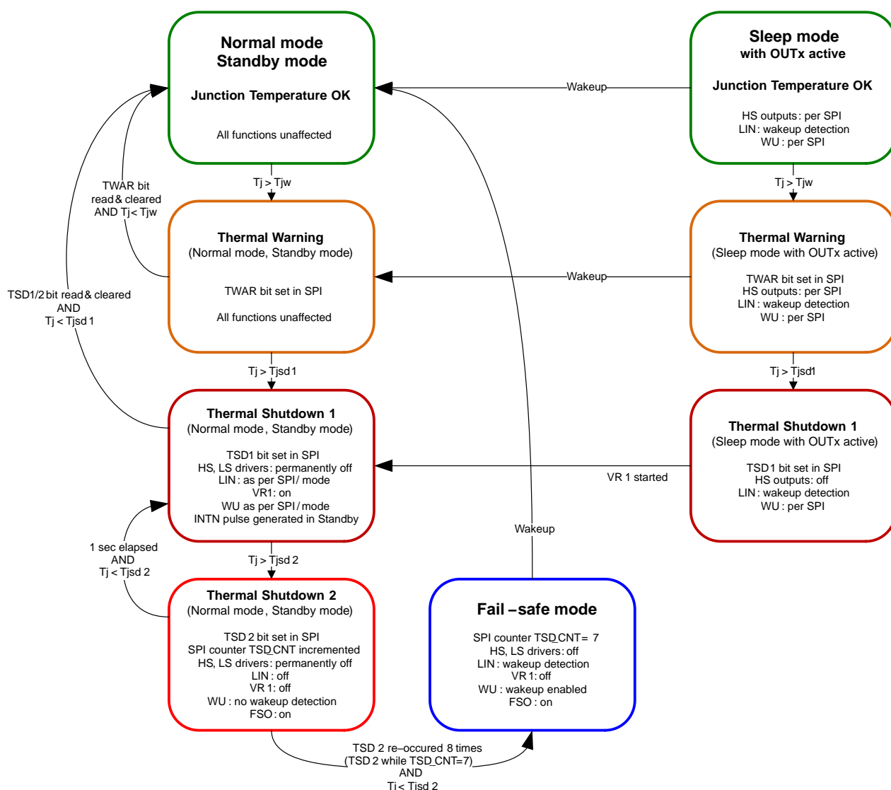
Figure 19. Thermal Protection
