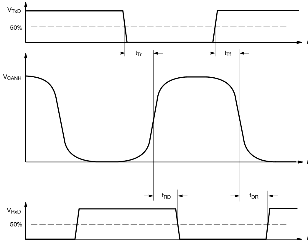
Figure 6. Input/Output Timing
