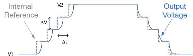
Figure 44. DVS in Forced PPWM Mode Diagram
