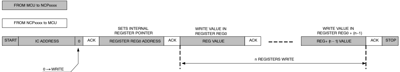
Figure 51. Write Sequence
