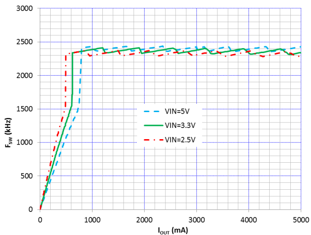
Figure 30. Switching Frequency vs I_{LOAD} and V_{IN} , V_{OUT} = 1.150\text{ V}
