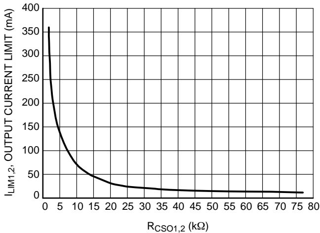
Figure 8. Output Current Limit vs. Rcs0 (Calculated Using E24 Series)
