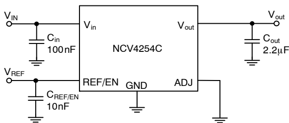
Figure 28. Adjust Version Application Circuit: High-Side Driver
