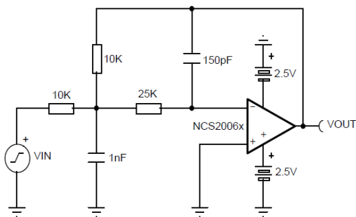
Figure 31. Second Order Active Low Pass Filter
