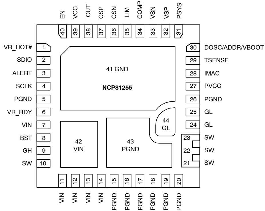
Figure 3. Pin Configuration
