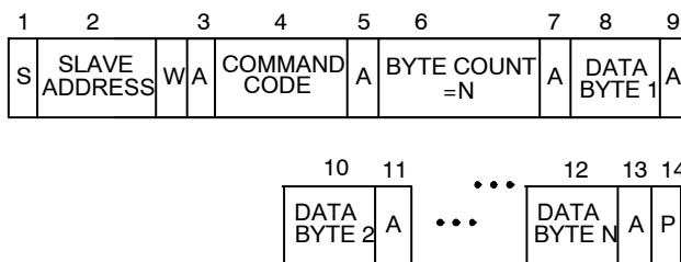
Figure 25. Block Write to a Register
