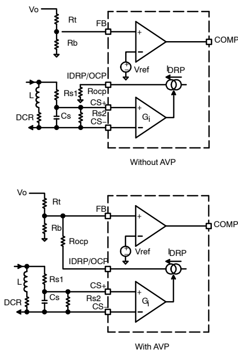
Figure 24. OCP Configuration
