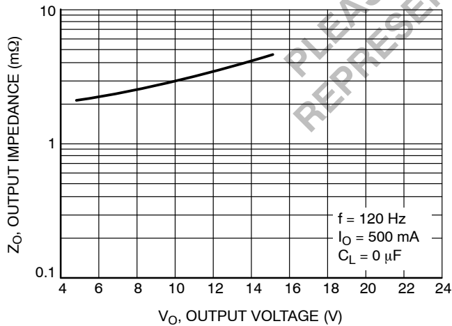
Figure 7. Output Impedance as a Function of Output Voltage
