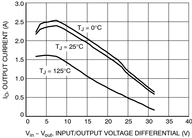
Figure 3. Peak Output Current as a Function of Input/Output Differential Voltage (NCP7805E)
