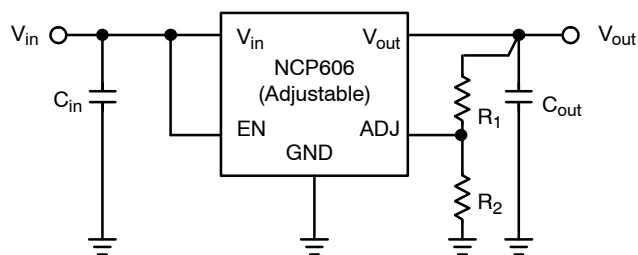
Figure 4. NCP606 Typical Application Circuit for Adjustable Version ( 1.25\text{ V} < V_{\text{out}} \leq 5.0\text{ V} )
