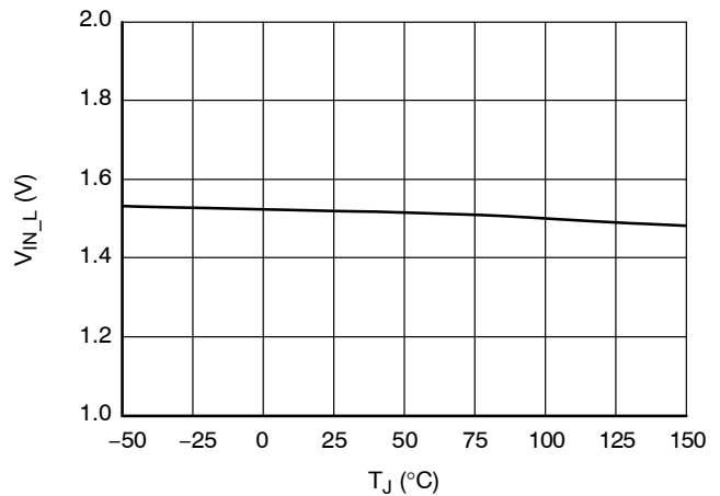
Figure 28. V IN_L V IN_L Input Threshold vs. Temperature
