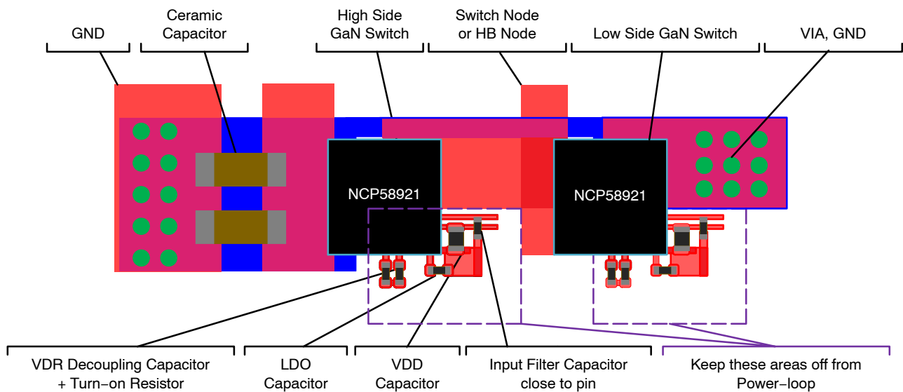
Figure 41. Half-Bridge Stage PCB Layout Recommendation
