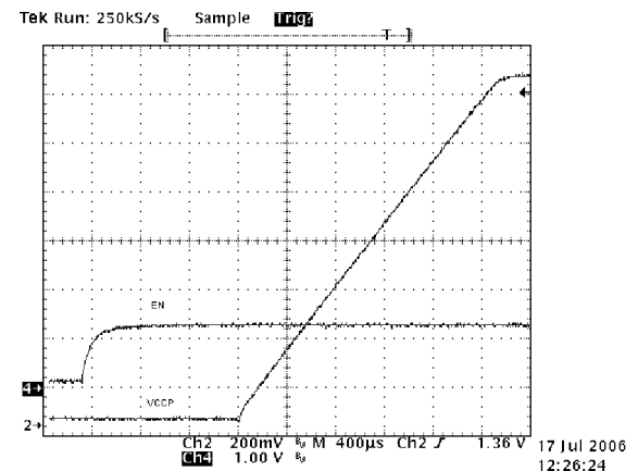
Figure 16. VR10 Legacy Startup
