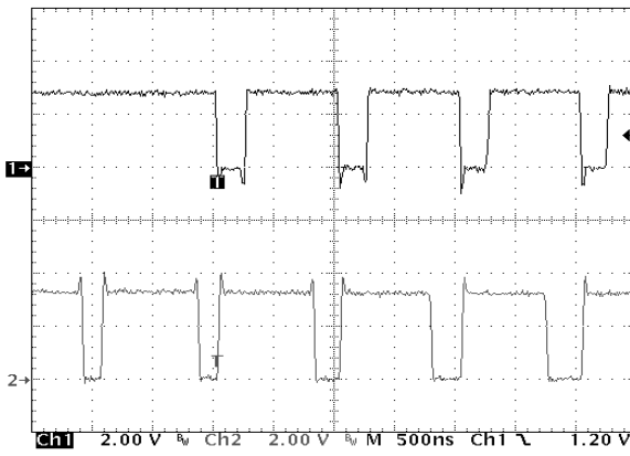
Figure 11. Transitional Period Switch Pins (LX1 and LX2) from Boost to Buck-Boost when V_{OUT} - V_{IN} is < than 375 mV
