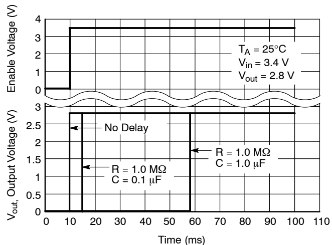
Figure 33. Delayed Turn-on
