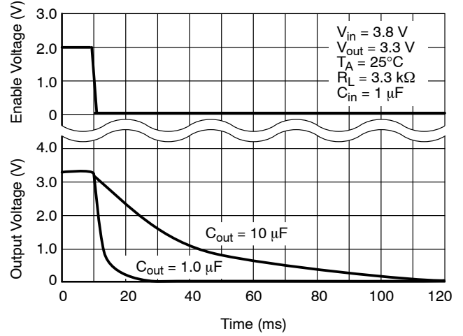
Figure 23. Turn-off Response
