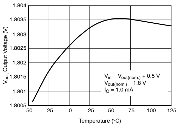
Figure 10. Output Voltage vs. Temperature
