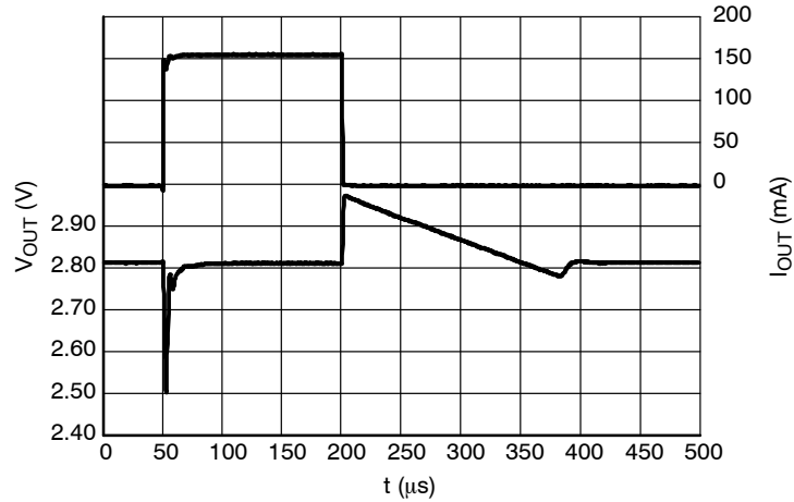
Figure 33. Load Transients, 2.8 V Version, I_{OUT} = 1 - 150 \text{ mA} , t_R = t_F = 0.5 \mu s , V_{IN} = 3.8 \text{ V}
