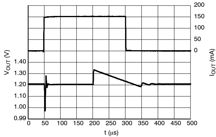
Figure 32. Load Transients, 1.2 V Version, I_{OUT} = 1 - 150 \text{ mA} , t_R = t_F = 0.5 \mu s , V_{IN} = 2.6 \text{ V}
