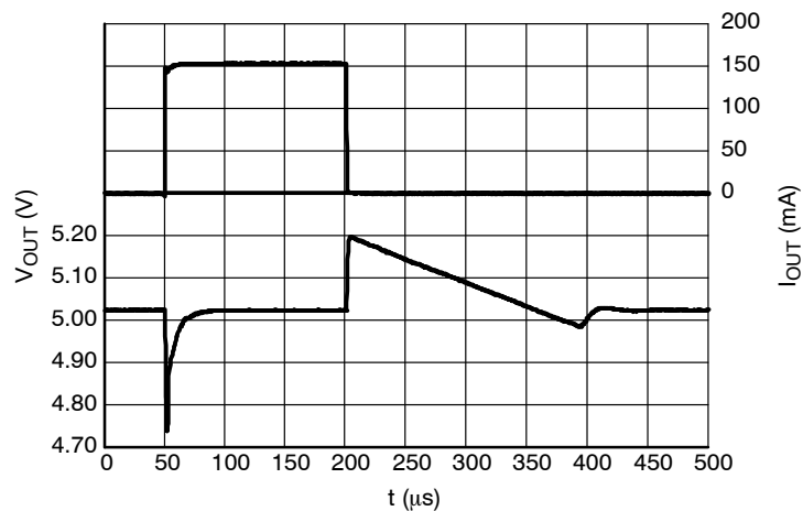
Figure 34. Load Transients, 5.0 V Version, I_{OUT} = 1 - 150 \text{ mA} , t_R = t_F = 0.5 \mu s , V_{IN} = 6.0 \text{ V}
