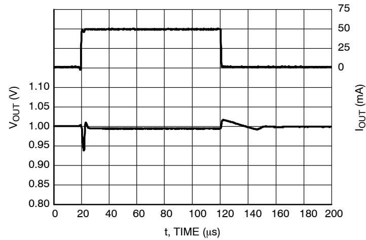
Figure 51. Load Transients, 1.0 V Version, I_{\text{OUT}} = 1 - 50 \text{ mA} , t_R = t_F = 0.5 \mu\text{s} , V_{\text{IN}} = 2.0 \text{ V} , \text{AE} = 0 \text{ V}
