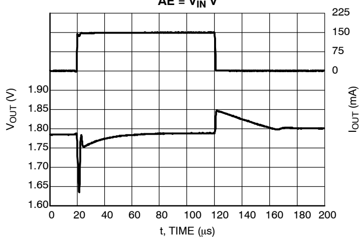
Figure 63. Load Transients, 1.8 V Version, I_{OUT} = 1 - 150 \text{ mA} , t_R = t_F = 0.5 \text{ } \mu\text{s} , V_{IN} = 2.8 \text{ V} , AE = 0 \text{ V}
