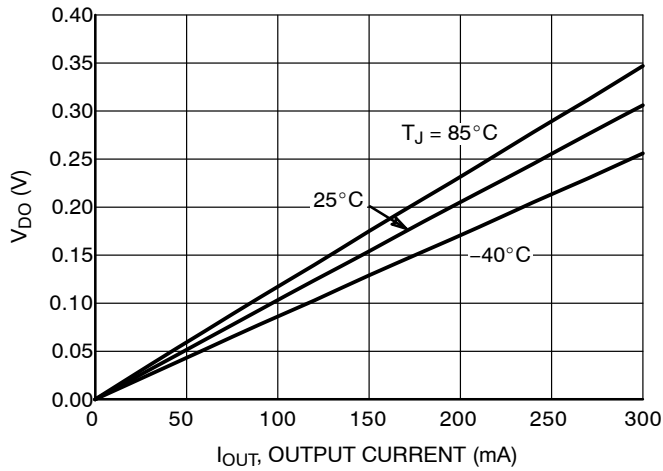
Figure 9. Dropout Voltage vs. Output Current 1.8 V Version
