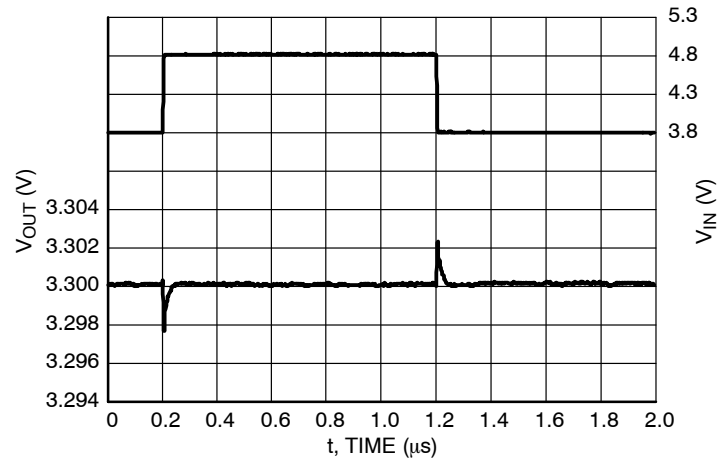
Figure 50. Line Transients, 3.3 V Version, t_R = t_F = 5 \mu\text{s} , I_{\text{OUT}} = 30 \text{ mA} , \text{AE} = V_{\text{IN}} \text{ V}
