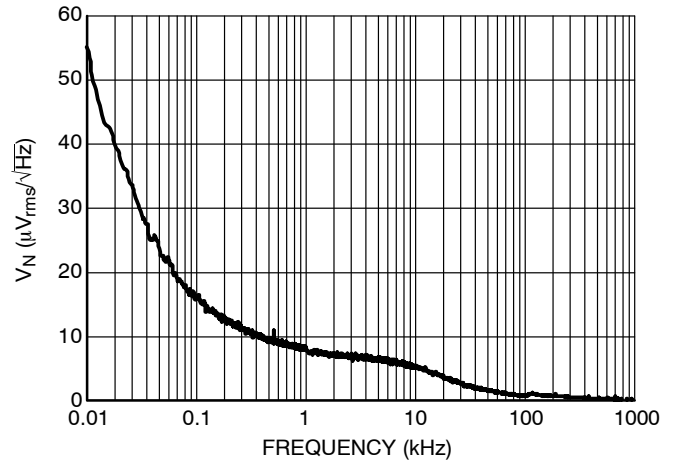
Figure 42. Output Voltage Noise, 3.3 V Version, V_{IN} = 4.3\text{ V} , I_{OUT} = 30\text{ mA}
