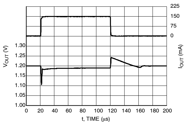
Figure 62. Load Transients, 1.2 V Version, I_{OUT} = 1 - 150 \text{ mA} , t_R = t_F = 0.5 \text{ } \mu\text{s} , V_{IN} = 2.2 \text{ V} , AE = V_{IN} \text{ V}
