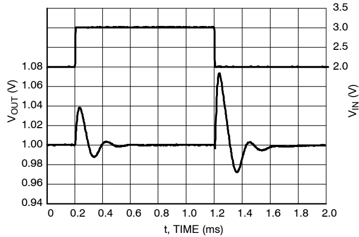
Figure 43. Line Transients, 1.0 V Version, t_R = t_F = 5\text{ μs} , I_{OUT} = 1\text{ mA} , AE = 0\text{ V}
