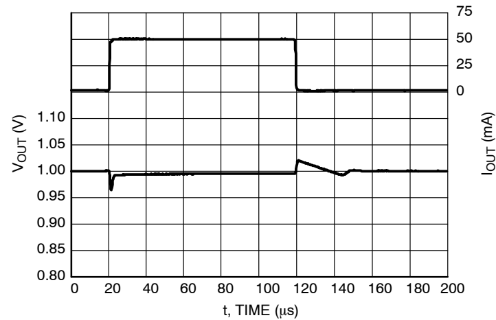
Figure 52. Load Transients, 1.0 V Version, I_{\text{OUT}} = 1 - 50 \text{ mA} , t_R = t_F = 0.5 \mu\text{s} , V_{\text{IN}} = 2.0 \text{ V} , \text{AE} = V_{\text{IN}} \text{ V}
