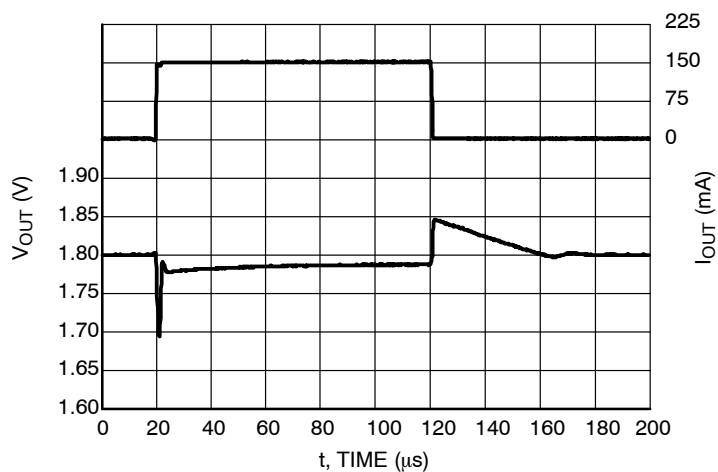
Figure 64. Load Transients, 1.8 V Version, I_{OUT} = 1 - 150 \text{ mA} , t_R = t_F = 0.5 \text{ } \mu\text{s} , V_{IN} = 2.8 \text{ V} , AE = V_{IN} \text{ V}
